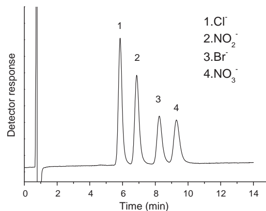
Fig. 1. Chromatogram obtained with a 150 mm × 3.9 mm column packed with SilprPy-H 2 O for the separation of chloride (1), nitrite (2), bromide (3), nitrate (4). Chromatographic conditions: mobile phase 2.5 mmol L -1 phthalic acid/2.4 mmol L -1 Tris, pH 4.2; flow rate: 1.5 mL min -1 ; injection volume: 20 µL; detector: non-suppressed conductivity.
